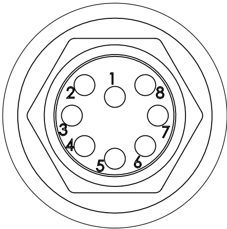
Single Connector:
