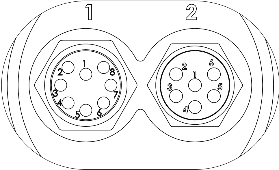
Dual Connectors:
