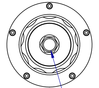
Brass female 8pin MCBH connector
